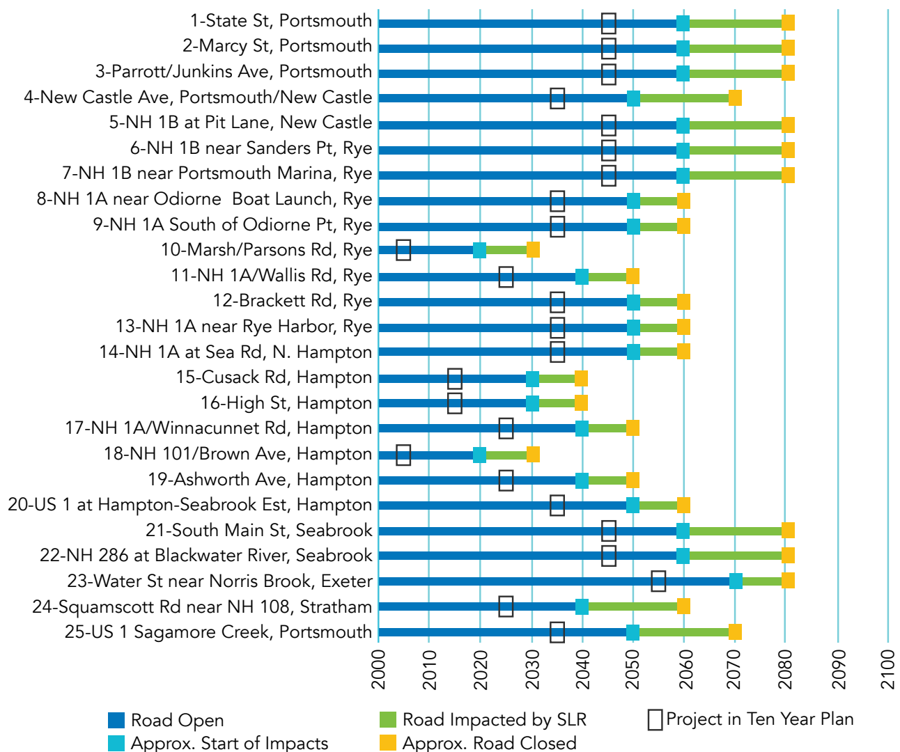
Figure 6.2: Planning Timeframes for Addressing Impacted Roadways
